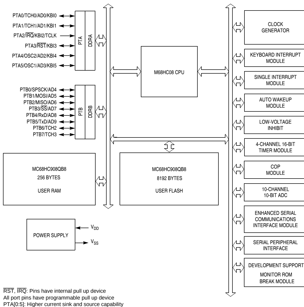
Figure 1-1. Block Diagram
