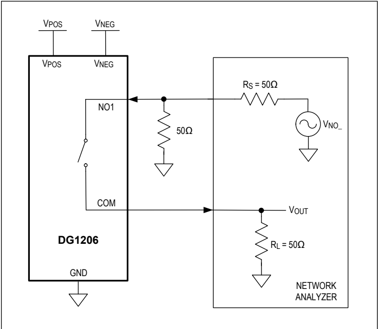
Figure 6. Off-Isolation (Similar Connection for DG1207)
