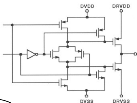
Figure 5. Pins 2-11 (D0-D9)
