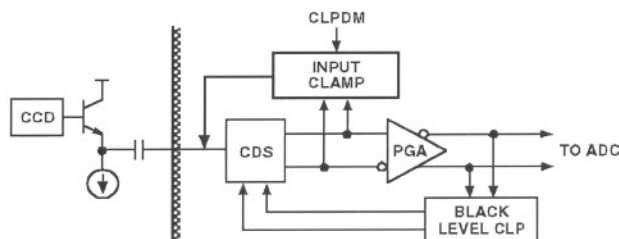
Figure 30. Input Clamp
