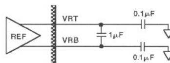
Figure 31. Reference Decoupling
