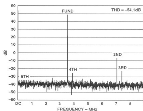
Figure 22. ADC-MODE at 18 MHz ( f_{IN} = 3.54 \text{ MHz} at -3 \text{ dB} )
