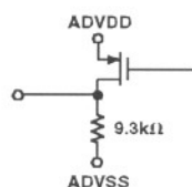
Figure 13. Pin 37 (CMLLEVEL)
