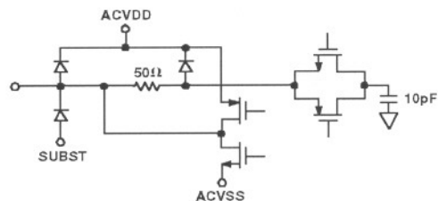
Figure 8. Pin 26 (DIN) and Pin 27 (PIN)
