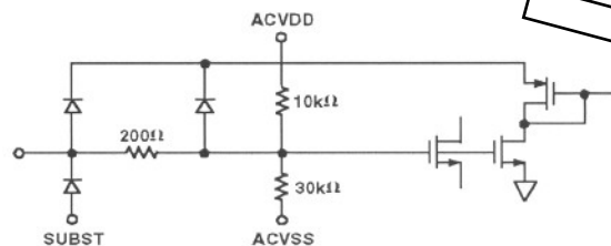
Figure 10. Pin 32 (CLPBYP)
