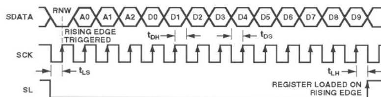
Figure 35. Serial WRITE Operation
