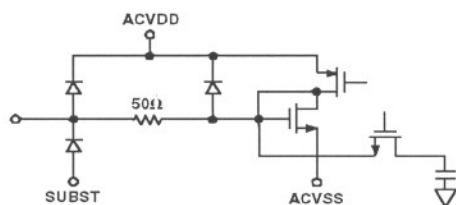
Figure 7. Pins 25, 28 (CCDBYP)
