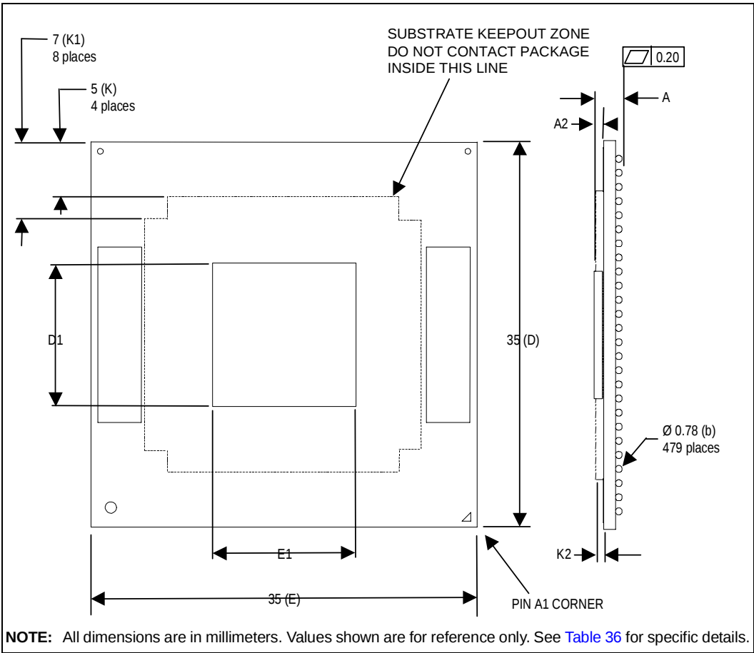
Figure 23. Micro FC-BGA Package – Top and Side Views
