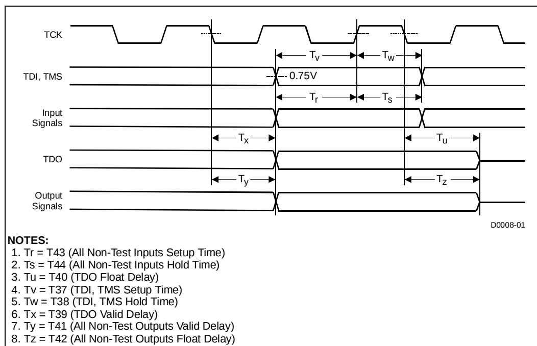
Figure 15. Test Timings (Boundary Scan)
