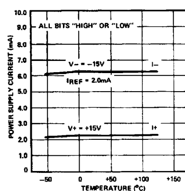
Figure 18. Power Supply Current vs. Temperature
