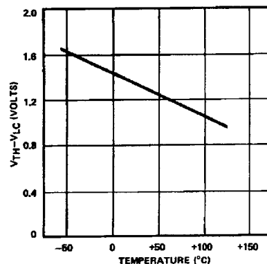
Figure 12. V_{TH}-V_{LC} vs. Temperature
