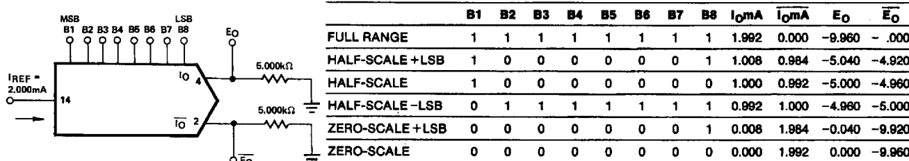
Figure 21. Basic Unipolar Negative Operation
