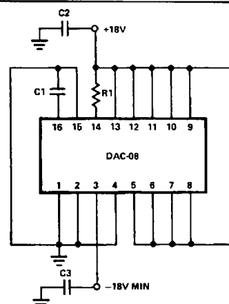
Figure 2. Burn-in Circuit
