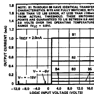
Figure 15. Bit Transfer Characteristics
