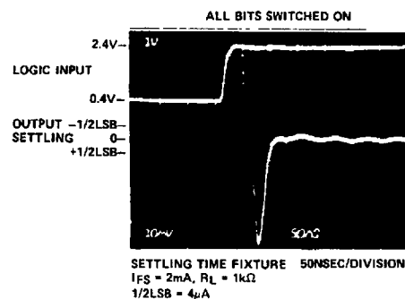
Figure 6. Full-Scale Settling Time
