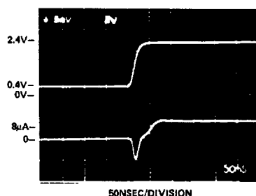
Figure 5. LSB Switching
