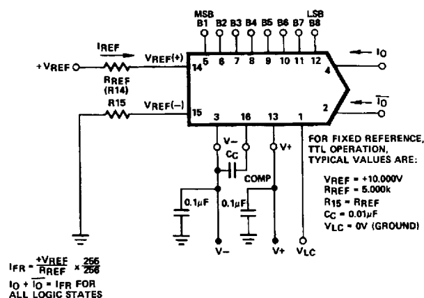
Figure 20. Basic Positive Reference Operation
