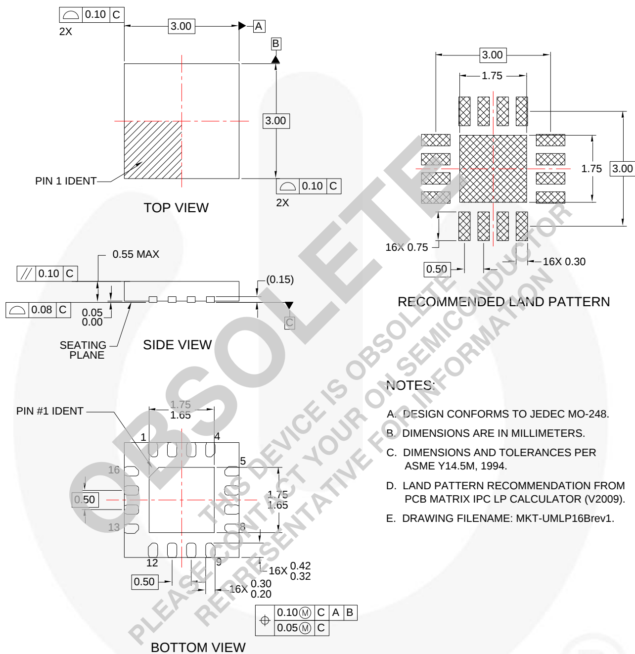
Figure 17. UMLP-16 Dimensions
