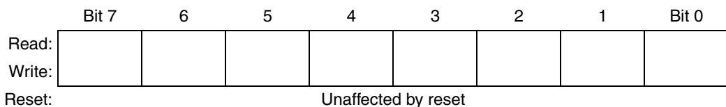
Figure 4-2. Accumulator (A)
