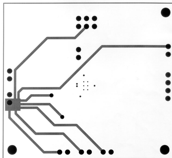
FIGURE 10. Recommended LD PC Board Layout: Inner Layer 2
