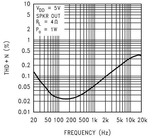
THD+N vs Frequency LM4855LQ
