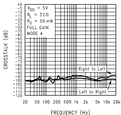
Channel Separation
