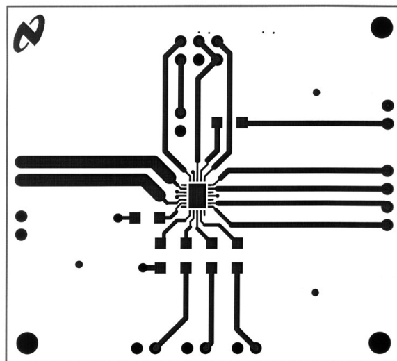
FIGURE 8. Recommended LD PC Board Layout: Top Layer
