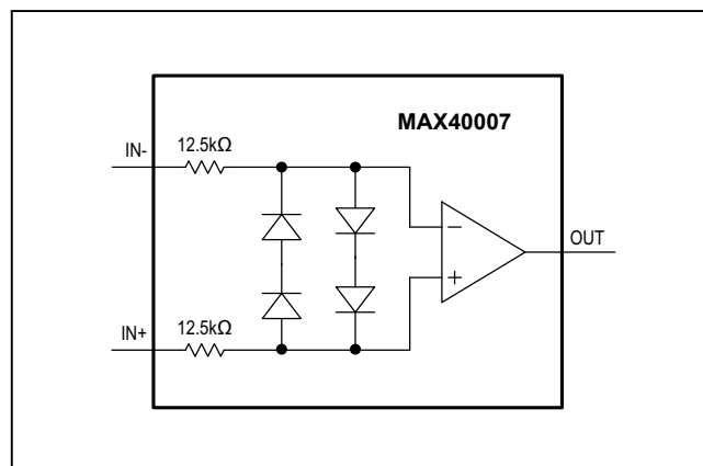
Figure 1. Input Protection Scheme
