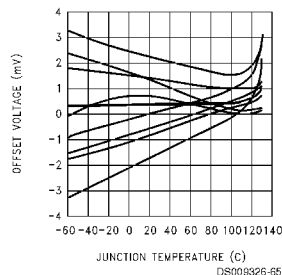
V_{OS} vs Junction Temperature on 9 Representative Units
