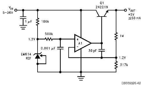
FIGURE 12. Simple Low Quiescent Drain Voltage Regulator. Total supply current approximately 320 \mu A , when V_{IN} = +5V .
