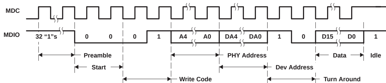
Figure 3–22. Management Interface Extended Space Write Timing
