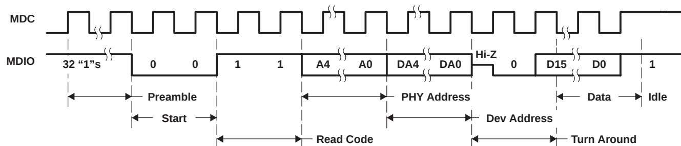
Figure 3–23. Management Interface Extended Space Read Timing
