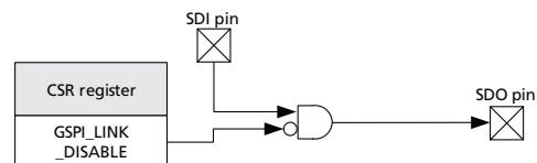
GSPI loop-through disable
