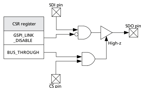
GSPI Bus-through enable
