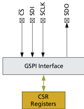
Figure 4-2: GSPI Interface Functional Block Diagram
