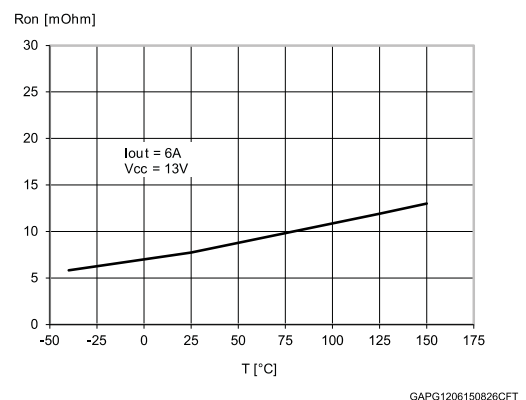
Figure 15: On-state resistance vs. Tcase
