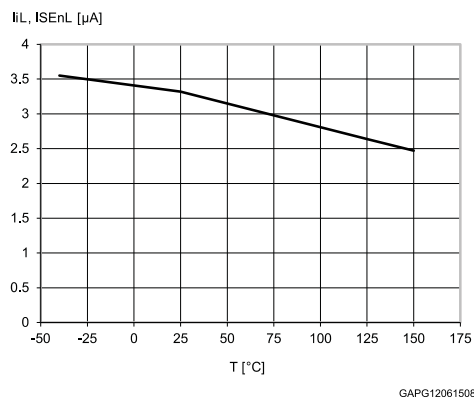
Figure 12: Low level logic input current
