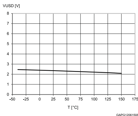
Figure 14: Undervoltage shutdown
