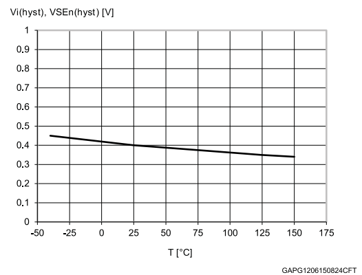
Figure 13: Logic Input hysteresis voltage
