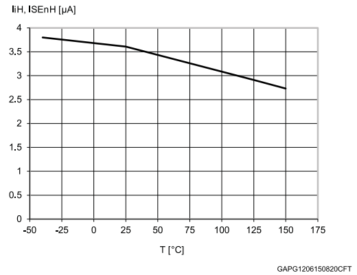
Figure 11: High level logic input current
