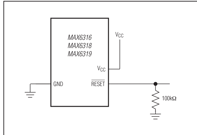
Figure 8. Ensuring \overline{RESET} Valid to V_{CC} = 0V on Active-Low Push/Pull and Bidirectional Outputs
