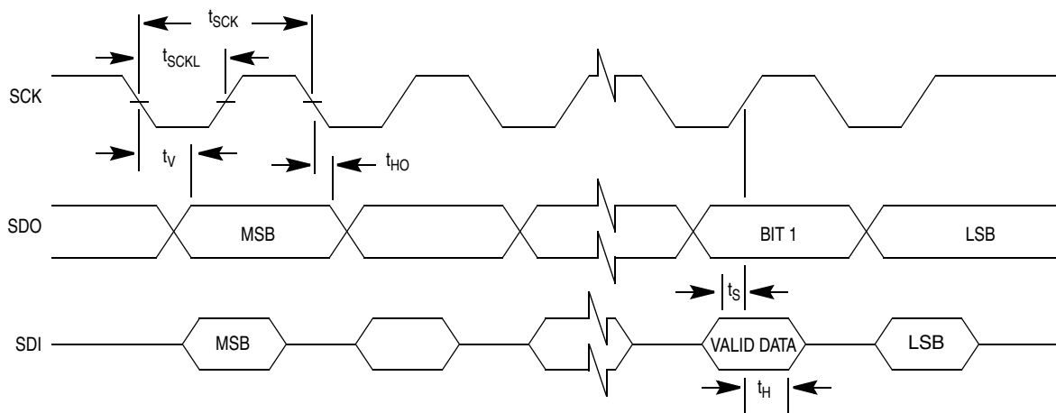
Figure 15-11. SIOPTiming Diagram
