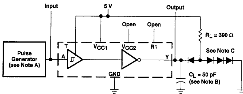
TEST CIRCUIT
