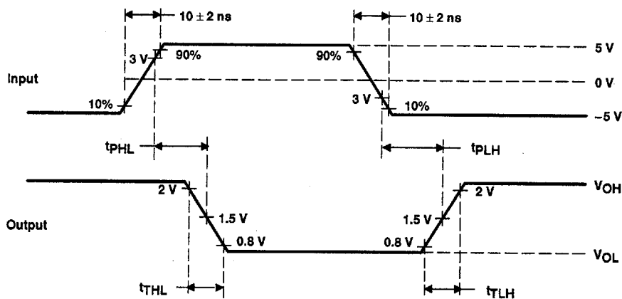
VOLTAGE WAVEFORMS
