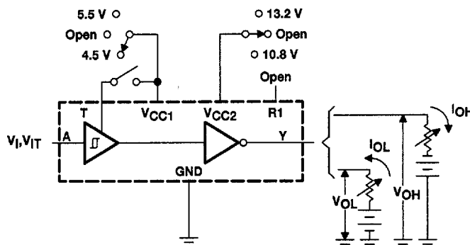
Figure 2. VIH, VIL, VIT+, VIT- → VOH, VOL
