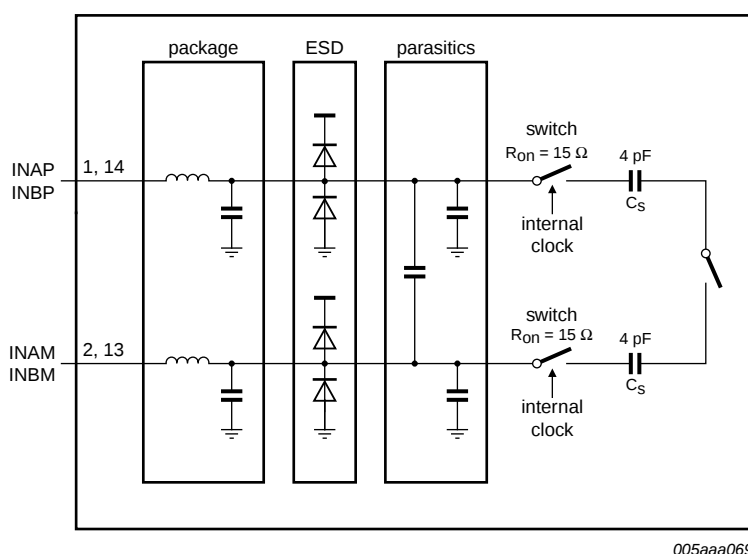
Fig 6. Input sampling circuit
