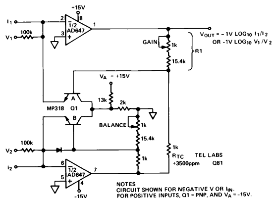
Figure 25. Log-Ratio Amplifier
