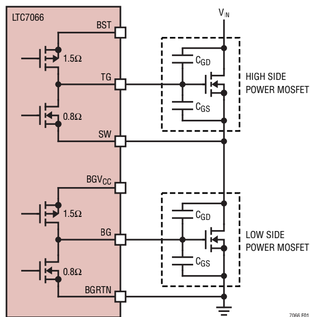
Figure 1. Simplified Output Stage in Half-Bridge Configuration
