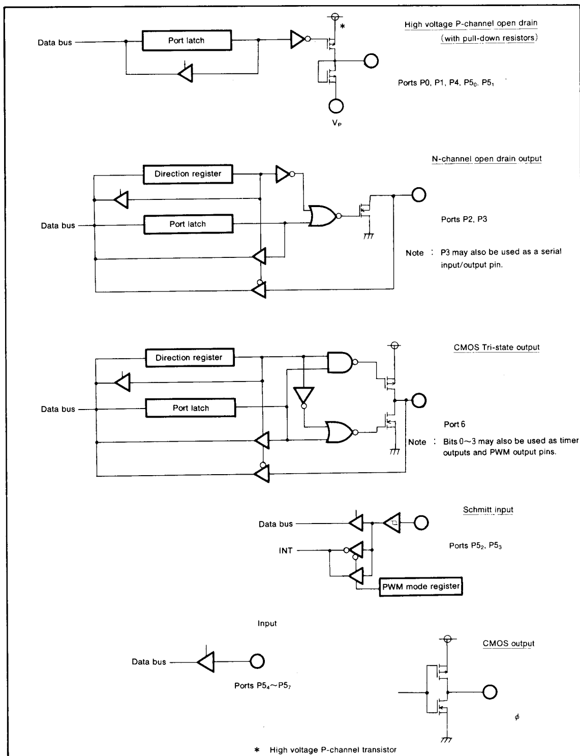
Fig.21 Block diagram of port P0~P6 (single-chip mode) and output format of φ
