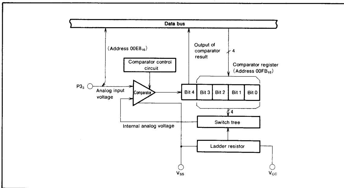
Fig.17 Comparator Circuit
