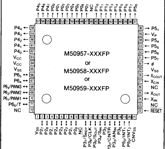
Outline 72P6
