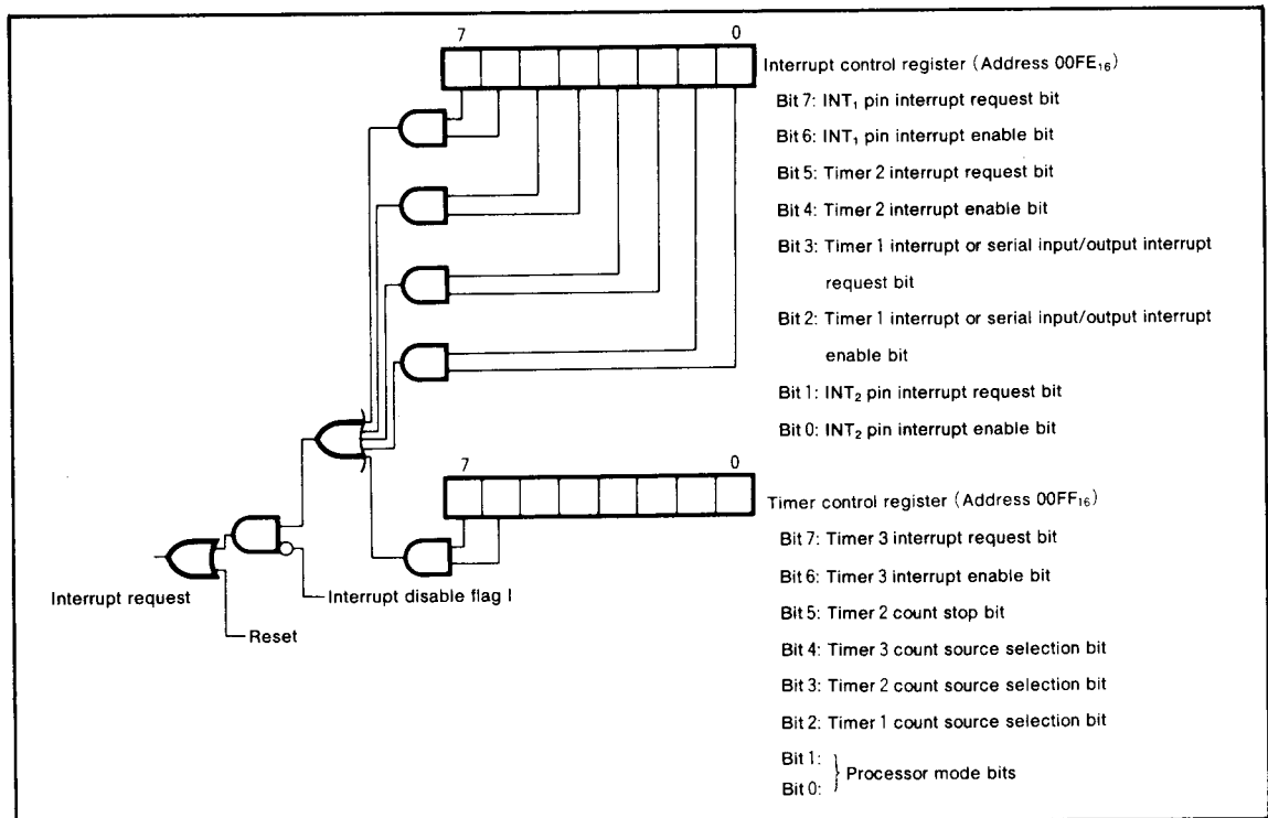
Fig.3 Interrupt control
