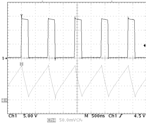
Figure 17. Continuous Current Mode (CCM) 1 SW, 5 V/div DC, 4 I_{SW} , 50 mA/div, DC, I_{OUT} = 15 mA
