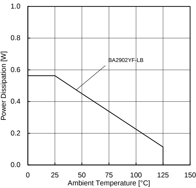
Figure 26. Derating Curve
