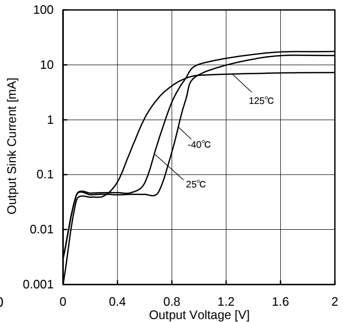
Figure 9. Output Sink Current vs Output Voltage (VCC=5V)
