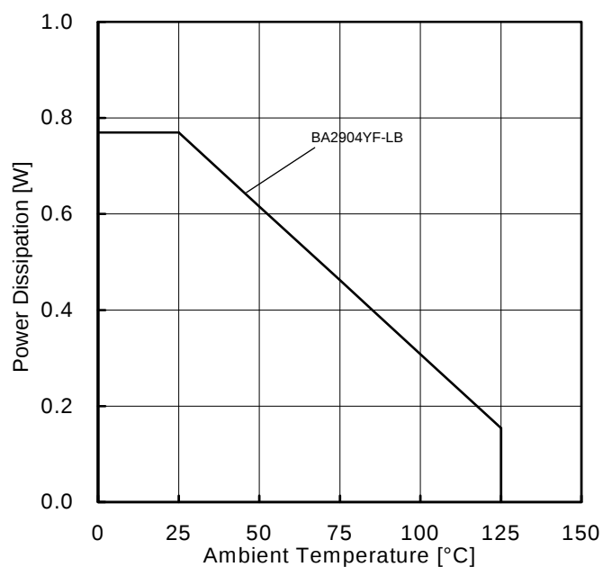
Figure 2. Derating Curve
