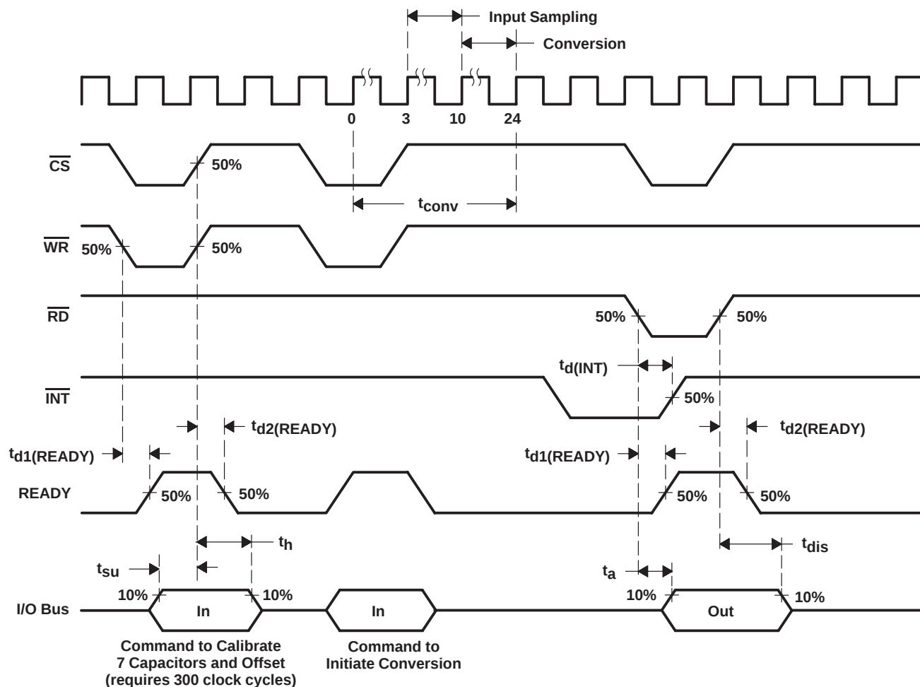
Figure 3. Timing Diagram
