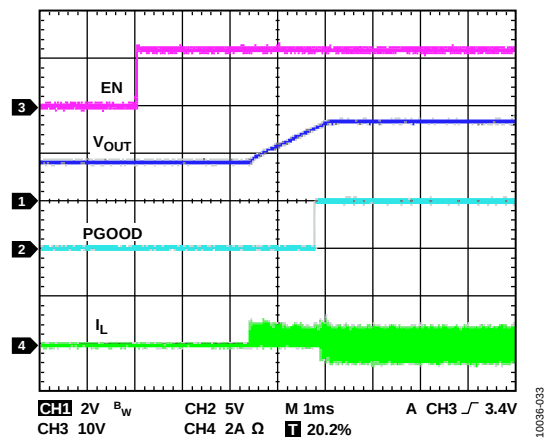
Figure 33. Soft Start with Precharged Output
