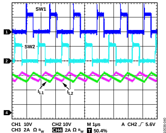
Figure 32. Dual Phase, Single Output, V_{OUT} = 3.3 V, I_{OUT} = 10 A
