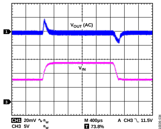
Figure 34. Line Transient Response, V_{IN} from 8 V to 14 V, I_{OUT} = 5 A
