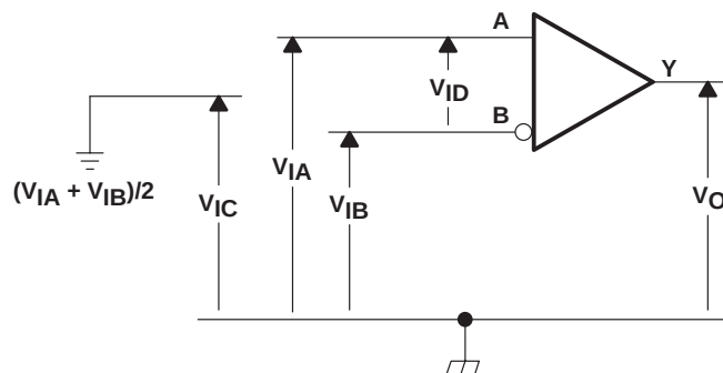
Figure 2. Voltage Definitions
