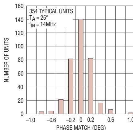
Channel to Channel Phase Matching
