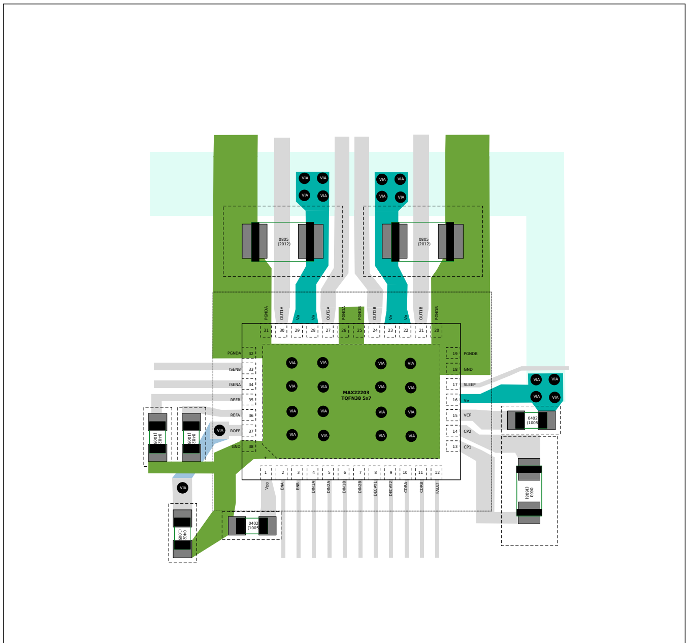
Figure 4. Recommended Layout
