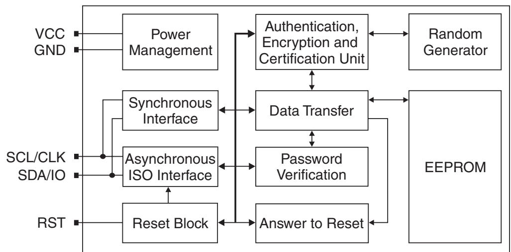
Figure 1. Block Diagram
