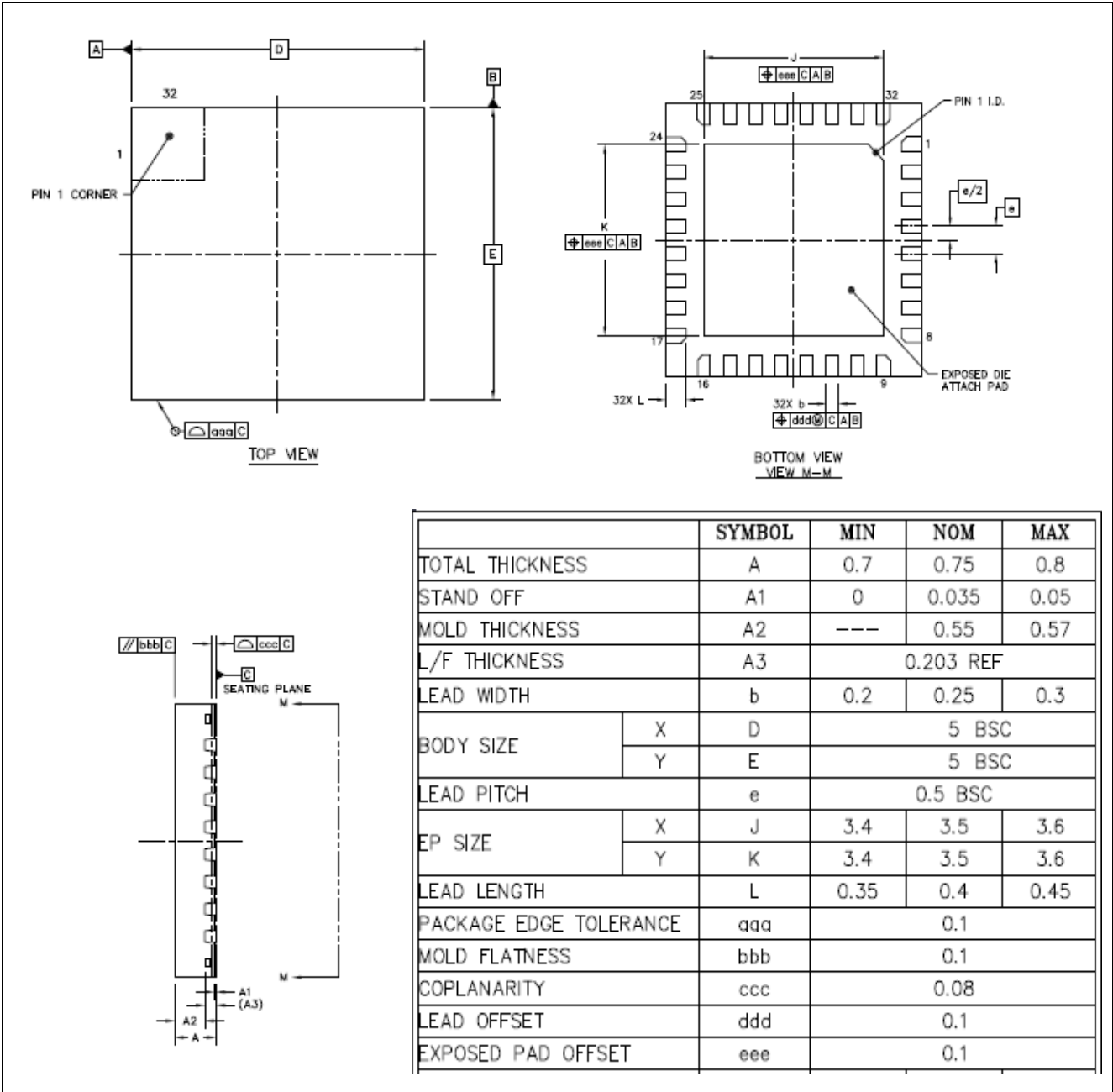
Figure 5 QFN 32-Lead Package
