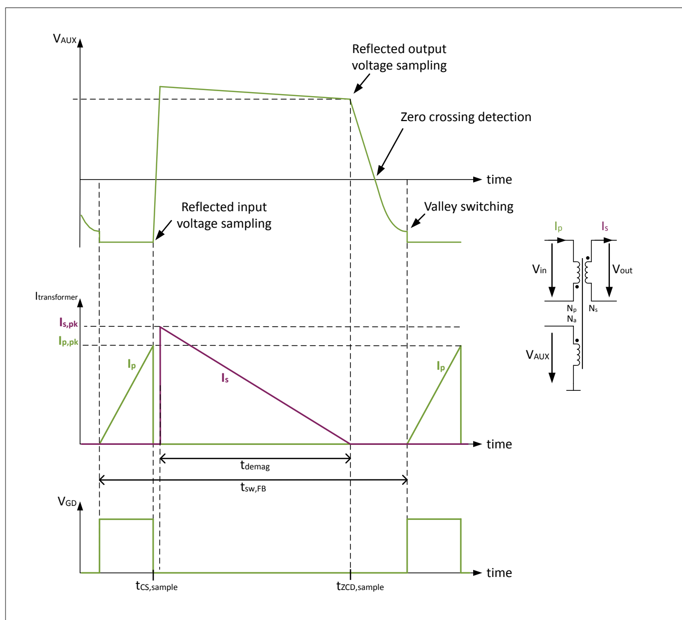
Figure 13 Flyback switching waveform example in QRM1
