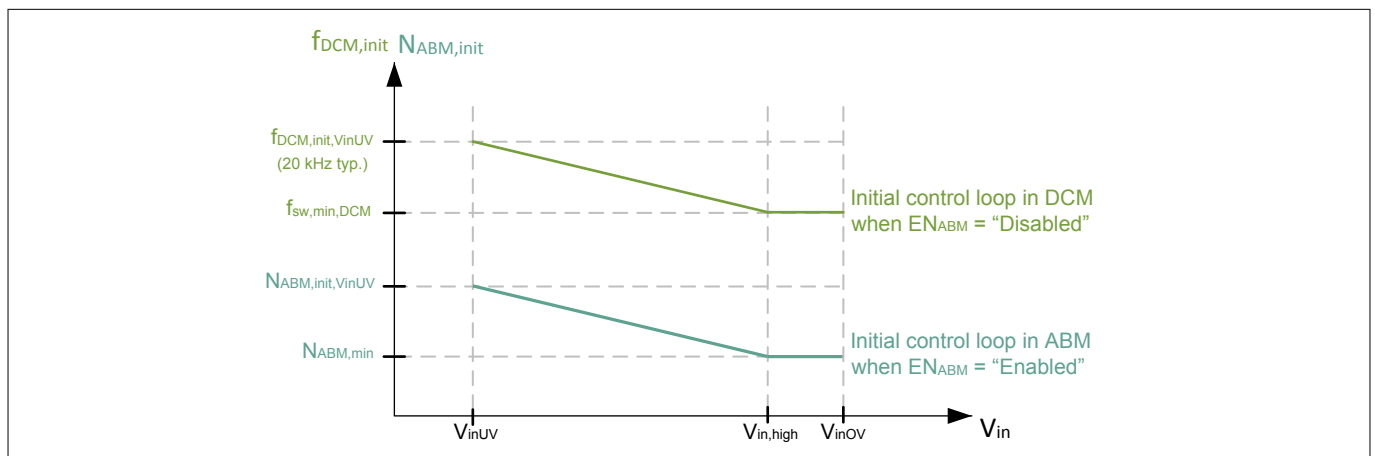
Figure 10 Adaptive control loop parameter initialization
