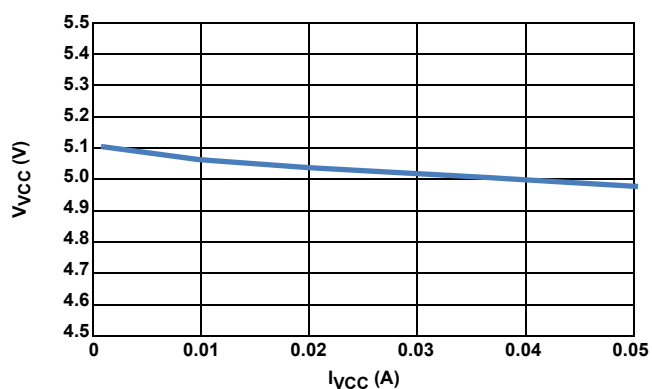
FIGURE 12. V_{VCC} vs I_{VCC}
