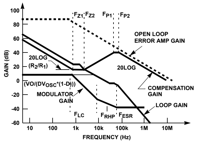
FIGURE 39. ASYMPTOTIC BODE PLOT OF CONVERTER GAIN
