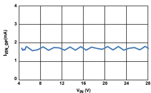
FIGURE 10. OPERATING CURRENT I_{VIN\_OP} vs V_{IN}
