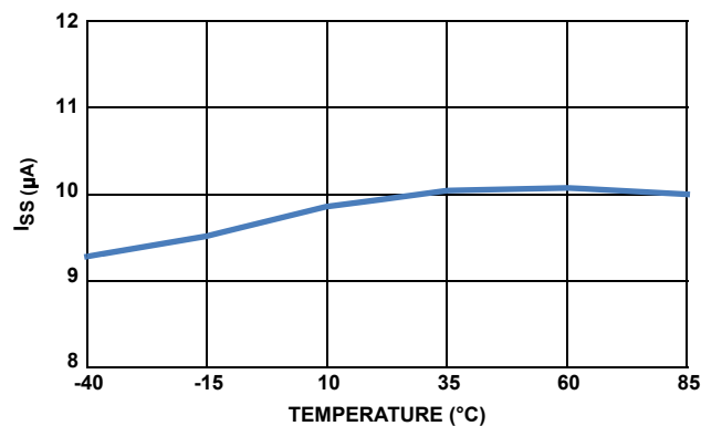
FIGURE 16. SOFT-START CURRENT, I_{SS} vs TEMPERATURE
