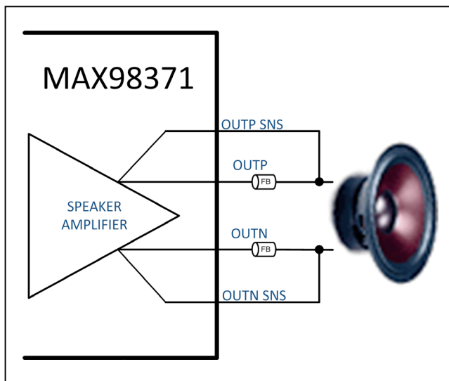
Figure 19. Typical Application Circuit with Ferrites Beads Used
