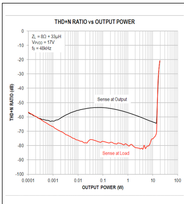
Figure 20. THD Performance Improvement Enabled by Remote Sensing
