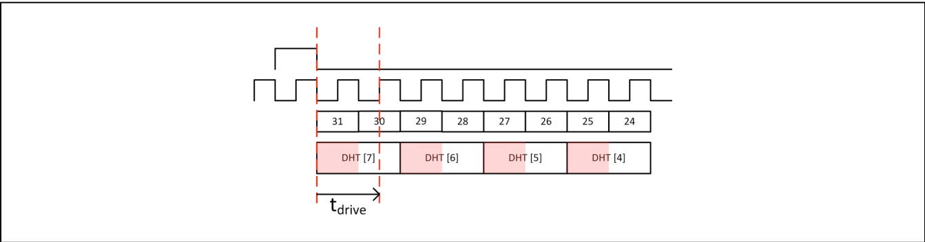
Figure 18. Double Data Drive illustration
