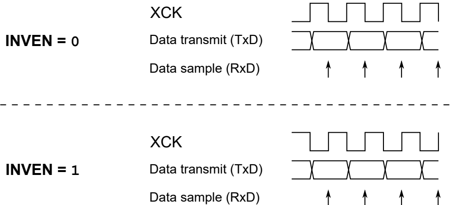
Figure 23-4. Synchronous Mode XCK Timing
