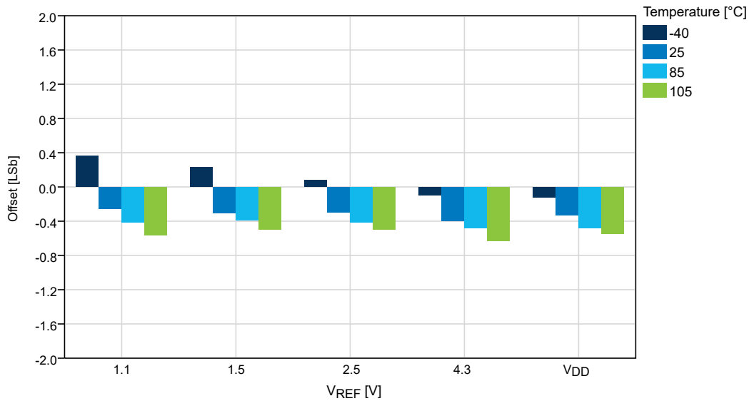
Figure 34-49. Offset Error vs. V_{REF} ( V_{DD} = 5.0V , f_{ADC} = 115 kps), REFSEL = Internal Reference
