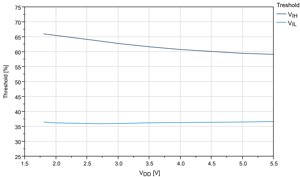
Figure 34-16. I/O Pin Input Threshold Voltage vs. V_{DD} ( T = 25^{\circ}\text{C} )
