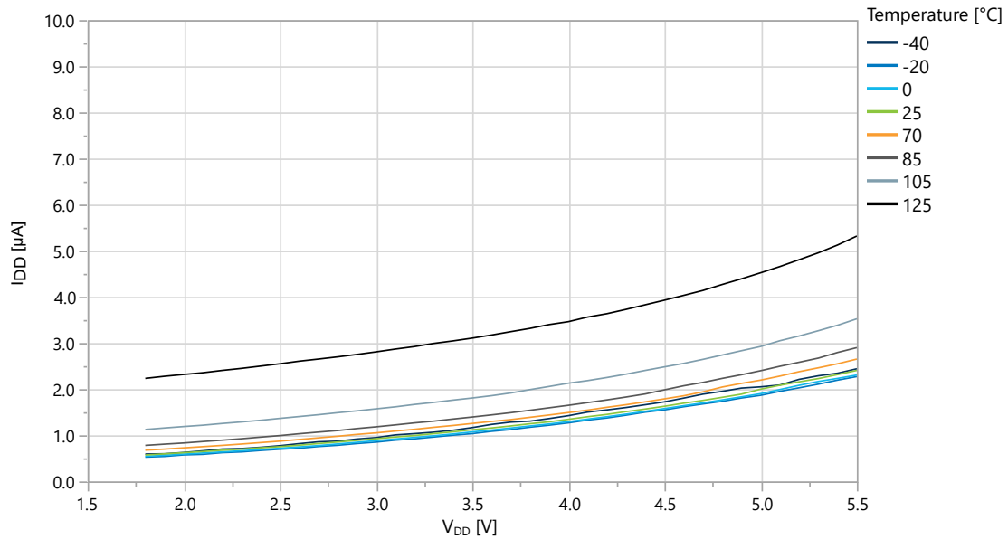
Figure 34-10. Standby Mode Supply Current vs. V_{DD} (RTC Running with Internal OSCULP32K)
