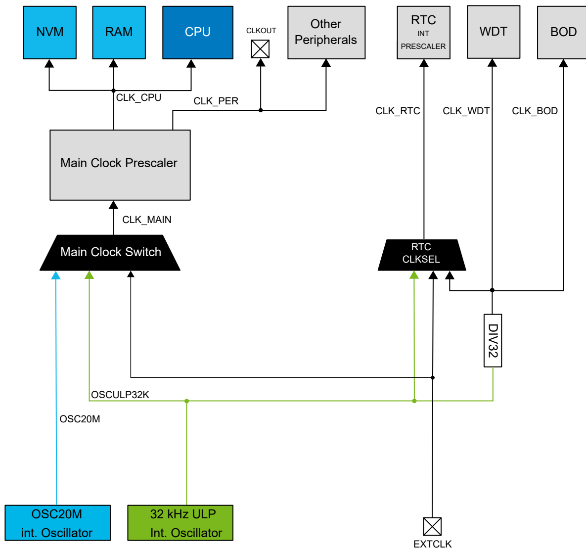
Figure 10-1. CLKCTRL Block Diagram
