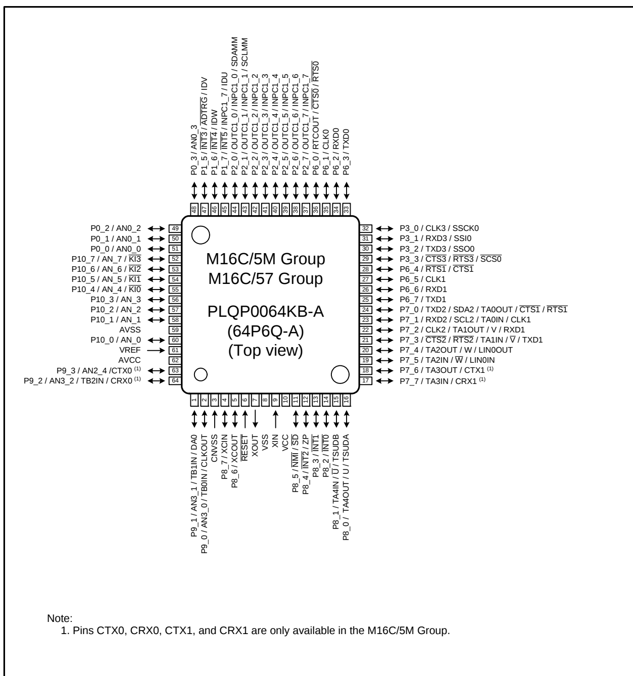
Figure 1.8 Pin Assignments for 64-Pin Package (Top View)
