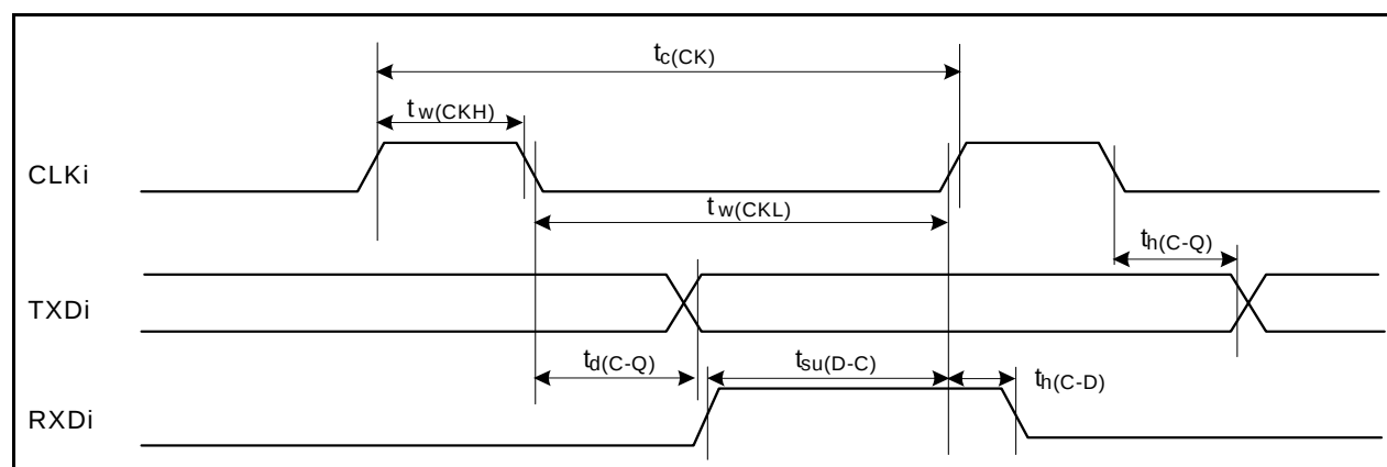
Figure 5.56 Serial Interface
