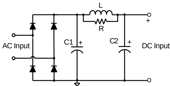
Figure 10: Input Filter
