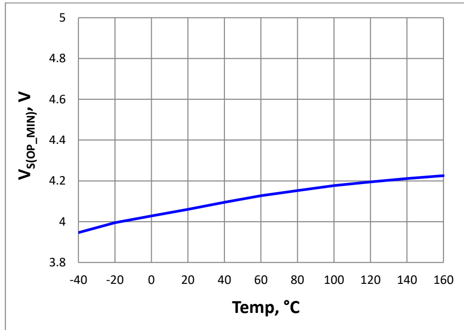
Figure 16. Minimum Functional Supply Voltage V_{S(OP\_MIN)} = f(T_J)
