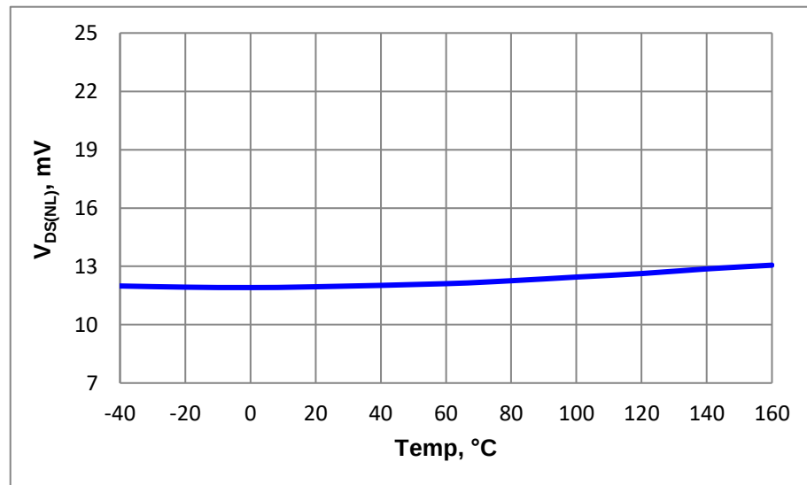
Figure 4. Output Voltage Drop Regulation, I_{OUT} = 30mA
