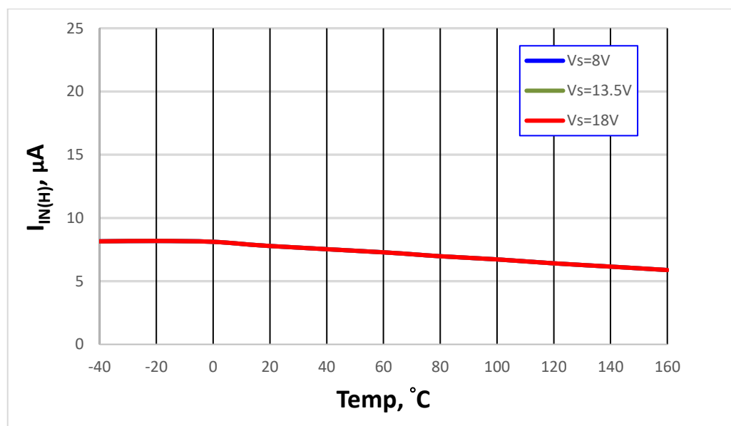
Figure 38. Input Current High Level I_{IN(H)} = f(T_J; V_S)
