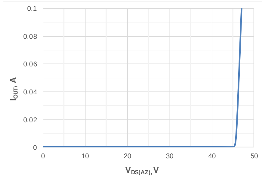
Figure 7. Typical Output Clamp Characteristic
