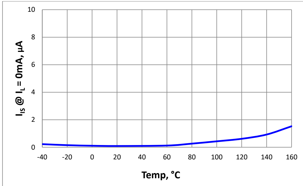
Figure 31. Current Sense at No Load I_{IS} = f(T_J)
