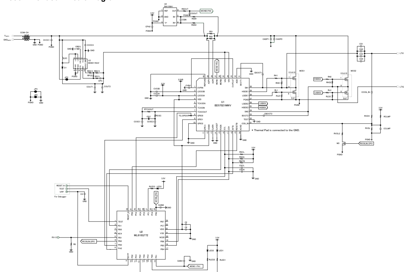
Figure 19. Typical application circuit diagram
