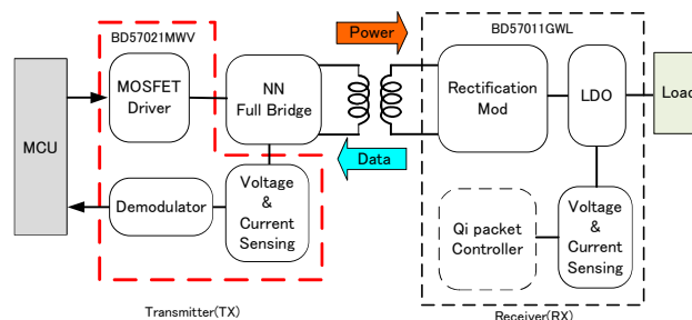
Figure 2. Product position in wireless power supply system
