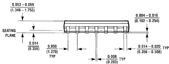
14-Pin SOIC NS Package Number MA14
