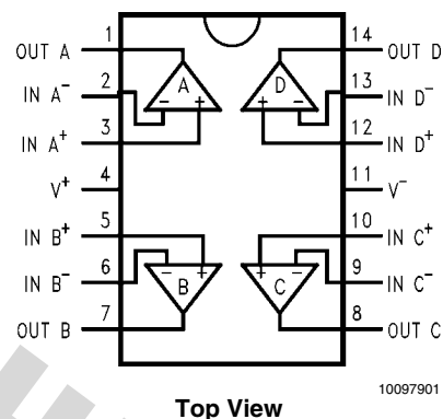
14-Pin TSSOP/SOIC
