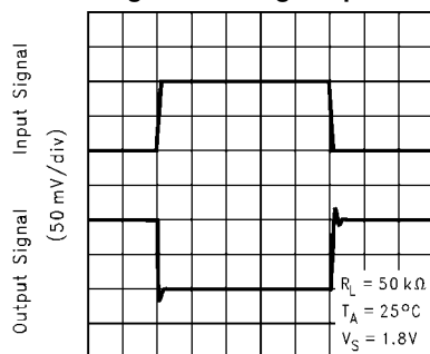
Small Signal Inverting Response
