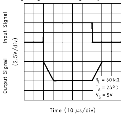
*Large Signal Inverting Response
