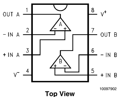
8-Pin MSOP/SOIC
