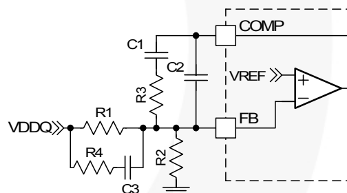
Figure 13. Compensation Network
