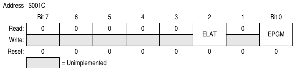
Figure 10-1. EPROM Programming Register (EPROG)
