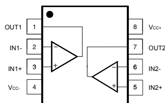
Figure 2. TSB712 pin connections (top view)
