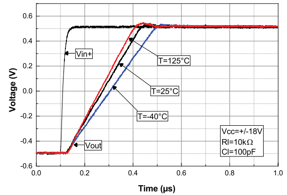
Figure 21. Positive slew rate at V_{CC} = 36\text{ V}
