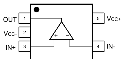
Figure 1. TSB711 pin connections (top view)
