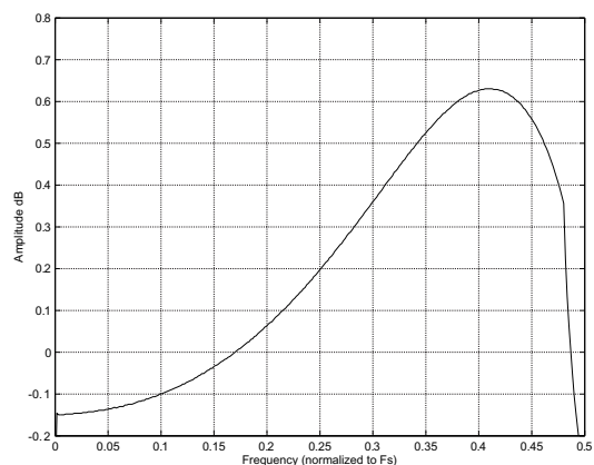
Figure 30. DAC Double-Speed Passband Ripple
