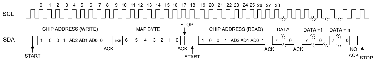
Figure 21. Software Mode Timing, I²C Read
