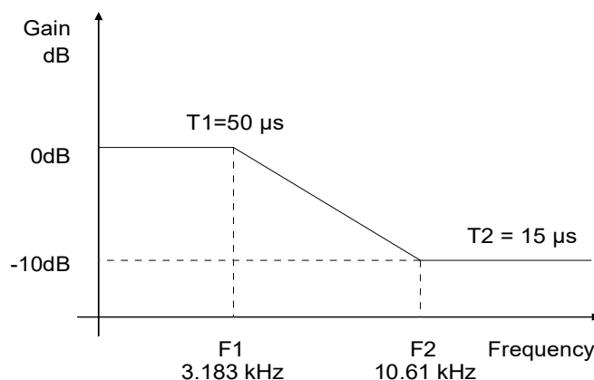
Figure 14. De-Emphasis Curve
