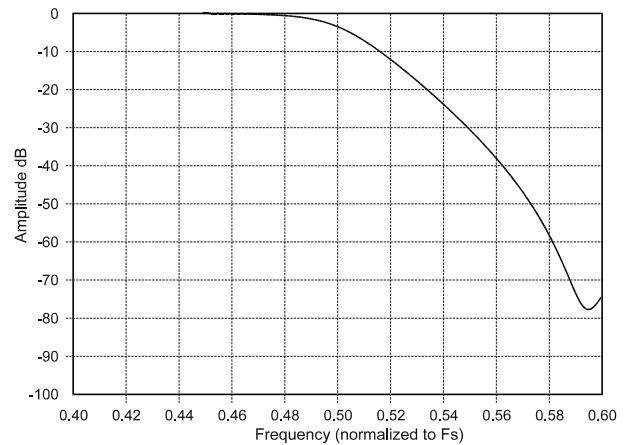
Figure 28. DAC Double-Speed Transition Band
