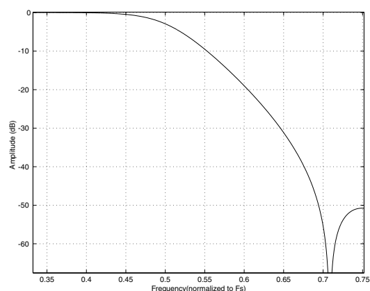
Figure 32. DAC Quad-Speed Transition Band
