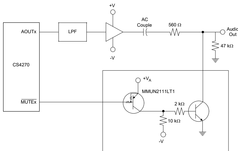
Figure 19. Suggested Active-Low Mute Circuit
