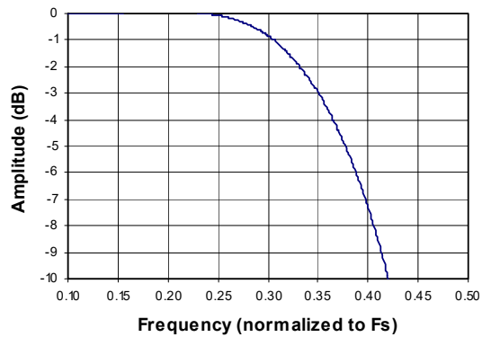
Figure 45. ADC Quad-Speed Transition Band (detail)
