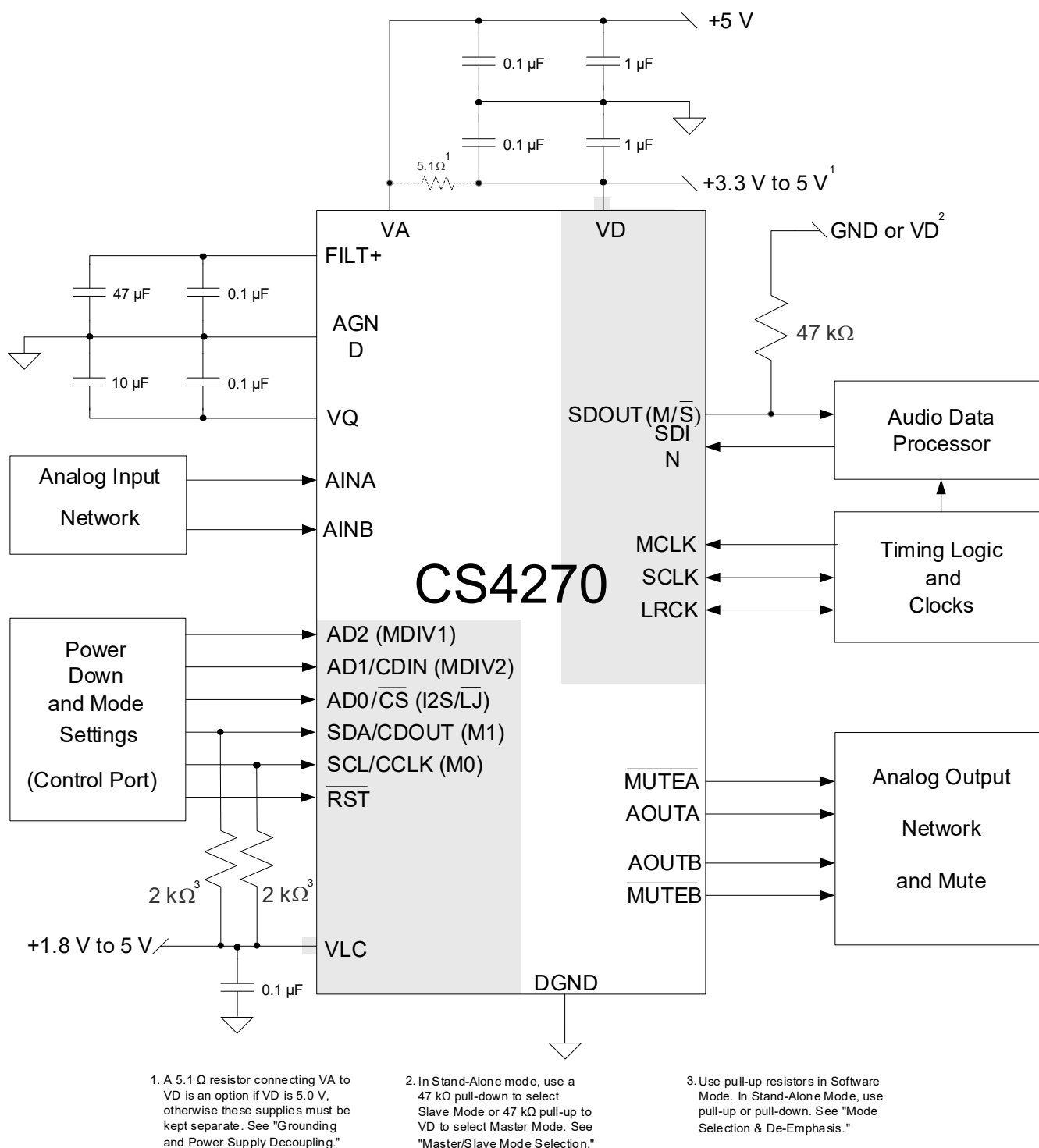
Figure 1. CS4270 Typical Connection Diagram
