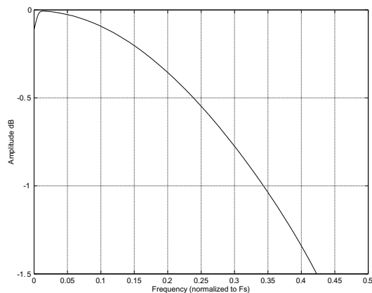
Figure 34. DAC Quad-Speed Passband Ripple
