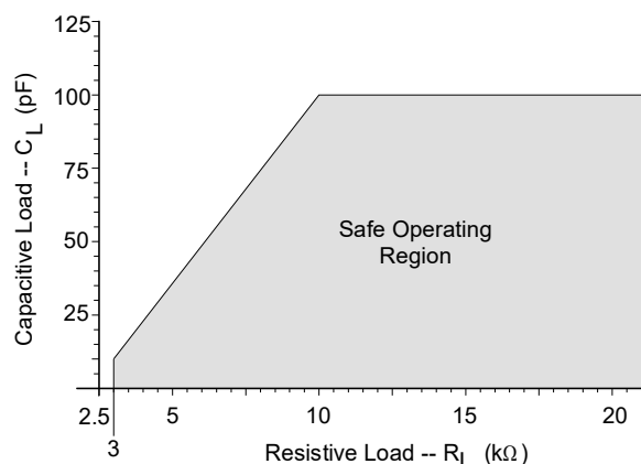
Figure 3. Maximum Loading
