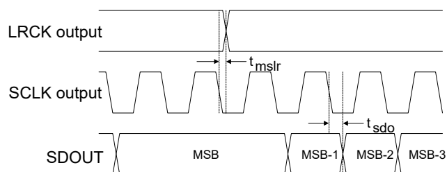
Figure 4. Master Mode, Left-Justified SAI
