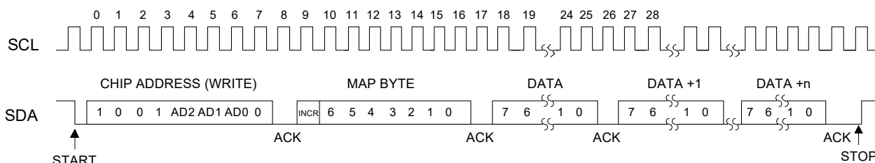
Figure 20. Software Mode Timing, I²C Write
