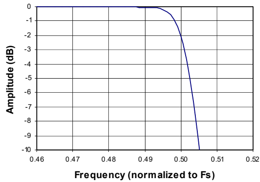
Figure 41. ADC Double-Speed Transition Band (detail)
