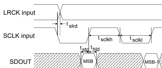
Figure 5. Slave Mode, Left-Justified SAI
