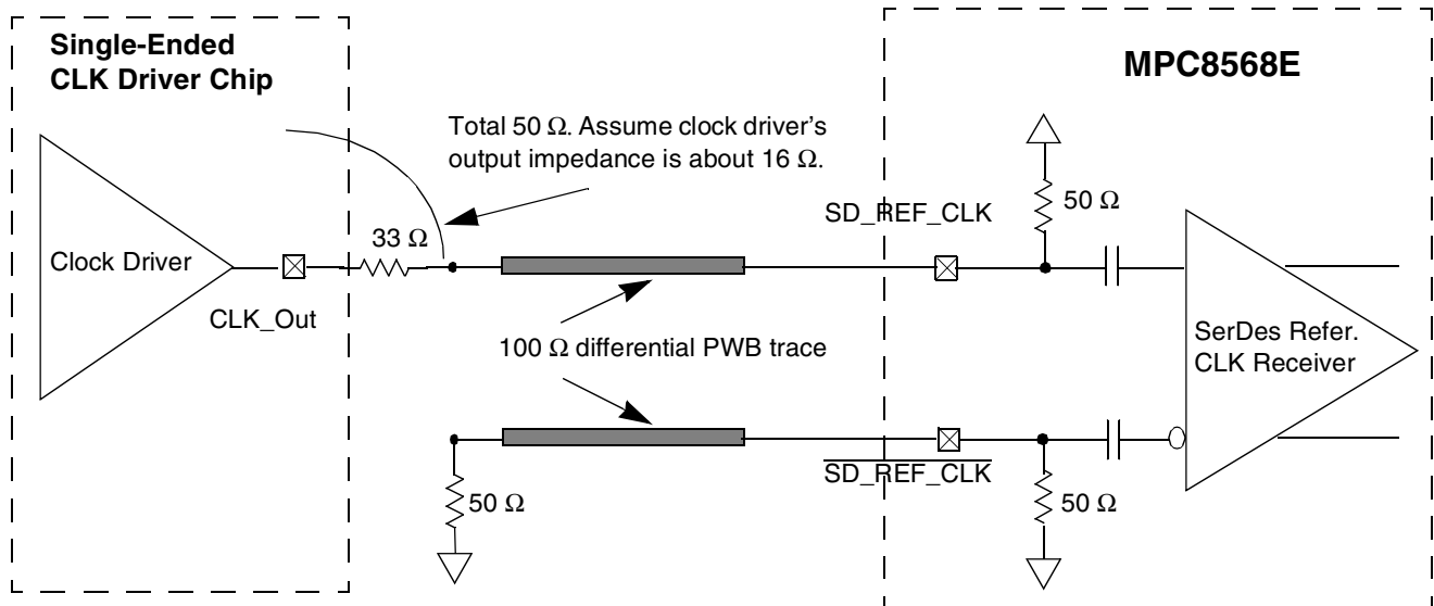
Figure 47. Single-Ended Connection (Reference Only)
