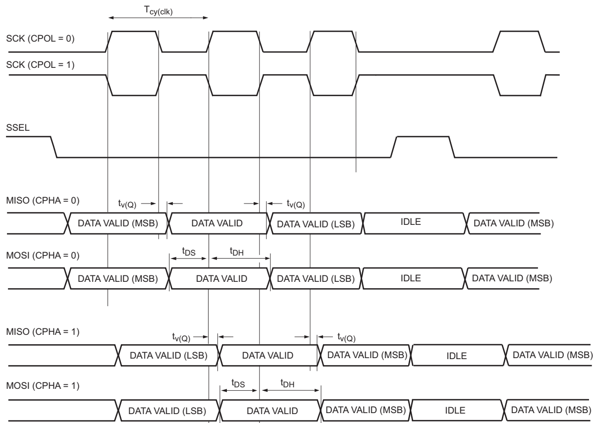
Fig 14. SPI slave timing
