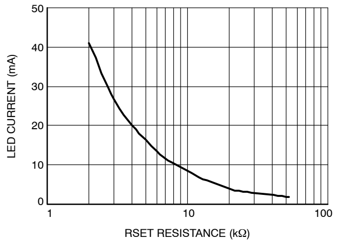
Figure 27. LED Current vs. RSET
