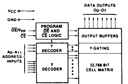
Figure 1. Block Diagram
