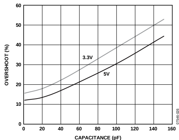
Figure 28. Small Signal Overshoot vs. Capacitive Load, 2 k \Omega in Parallel with Capacitive Load
