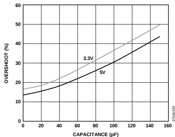
Figure 27. Small Signal Overshoot vs. Capacitive Load, 600 \Omega in Parallel with Capacitive Load
