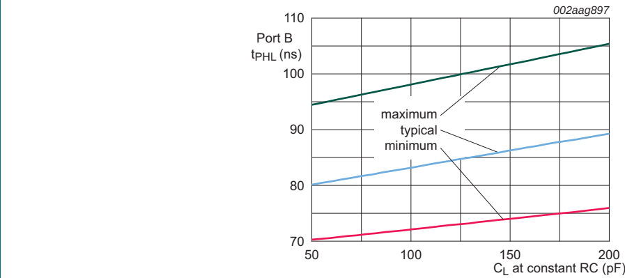
Fig 12. Nominal port B t_{PHL} with load capacitance at constant RC
