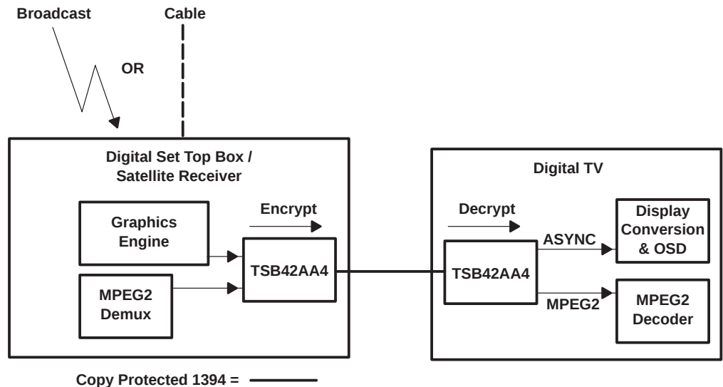
Figure 2–2. Graphics Overlay From Digital STB to DTV
