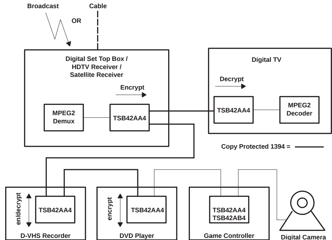
Figure 2–1. Home Entertainment System Interconnect With Content Protection
