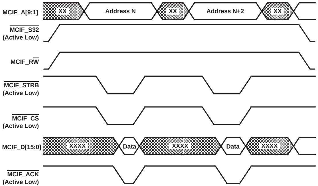
Figure 3-2. 16-Bit Read
