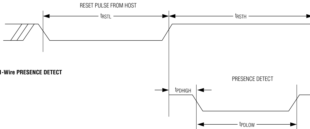
1-Wire RESET PULSE
